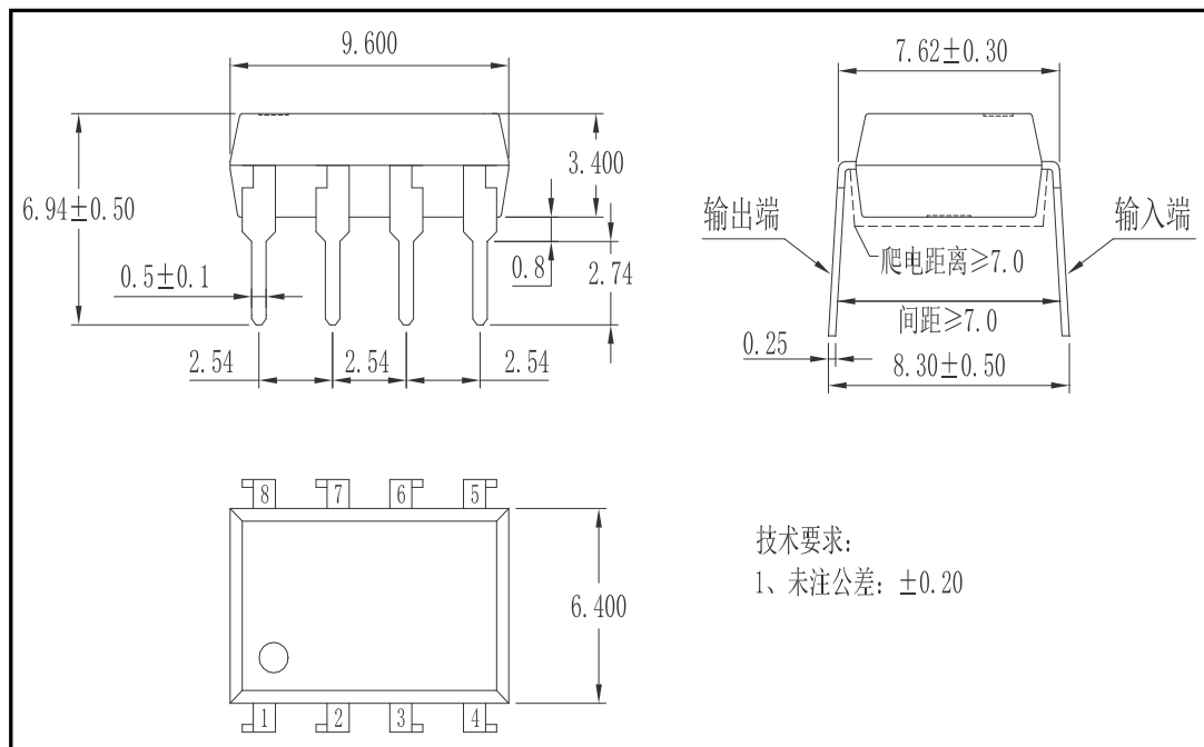
图 3 HSSR-DA09 外形尺寸 Figure 3- The dimensions of HSSR-DA09
