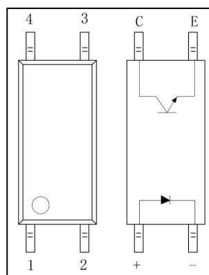
图 2 电原理图 Figure 2-Schematic
